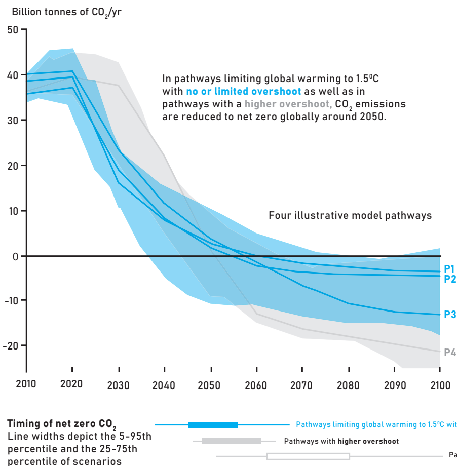
Figure 2. Global Emission Pathways. Source: IPCC (2018).
