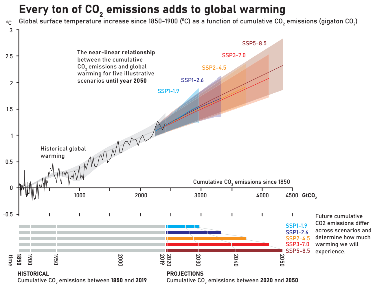
Figure 1. A near-linear relationship between cumulative CO 2 emissions and the increase in global surface temperature. Source: IPCC (2021).
